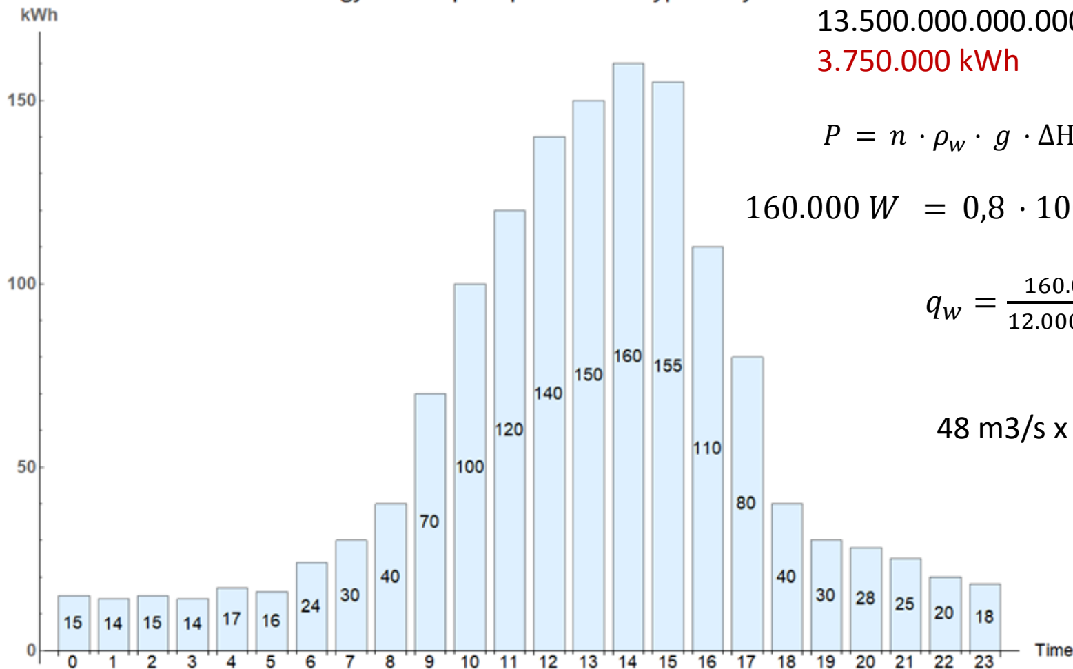
Energy Consumption per hour of a typical day
