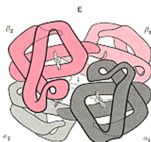
QUATERNARY STRUCTURE
