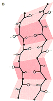
\beta sheet
